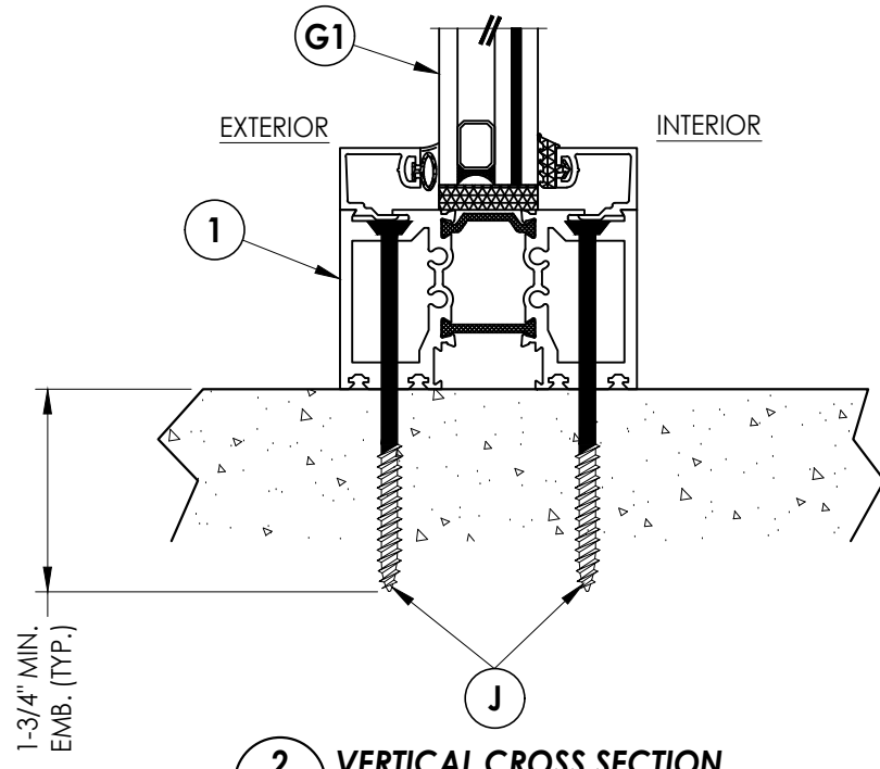
2 9 VERTICAL CROSS SECTION
