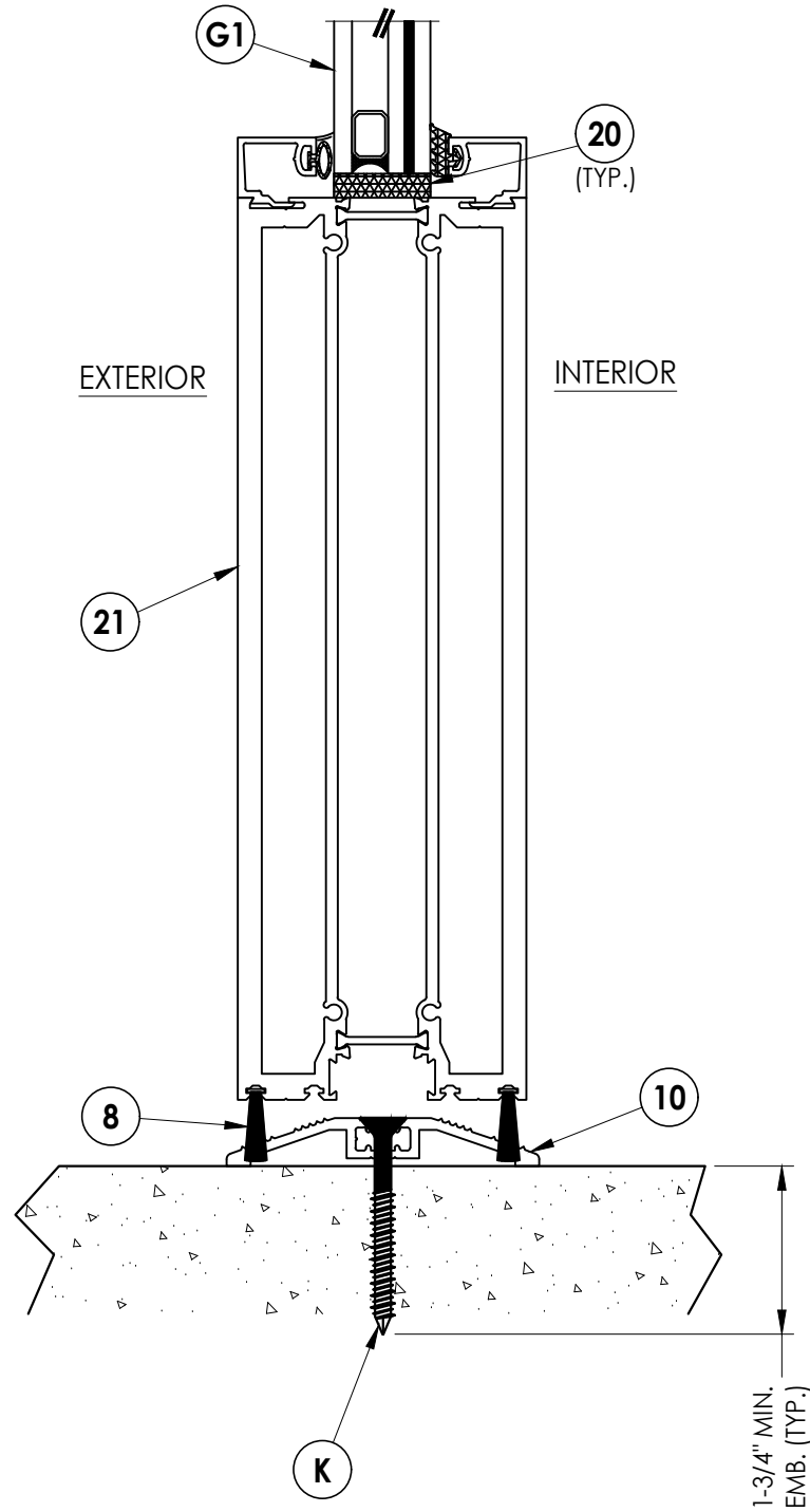
3 9 VERTICAL CROSS SECTION
