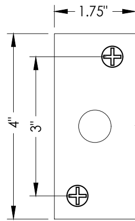
PIVOT HINGE FLOOR PLATE PLAN VIEW
